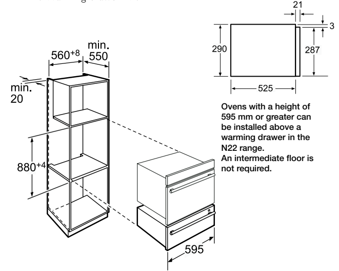
N22H40 Warming drawer 290mm
